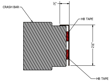
SECTION A-A 2 1/8" X 16" RECTANGULAR CRASH BAR COVER
