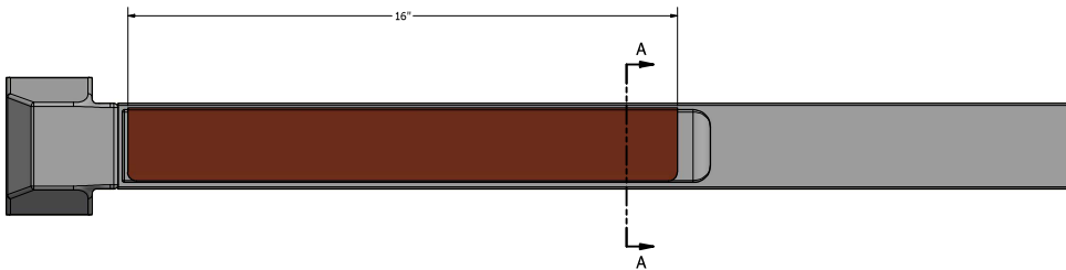
ELEVATION 2 1/8" X 16" RECTANGULAR CRASH BAR COVER
